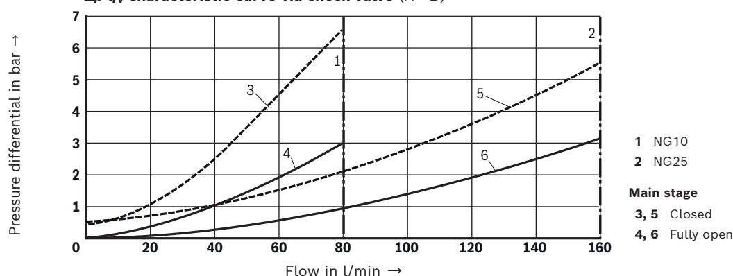
\Delta p-q_v characteristic curve via check valve (A→B)
