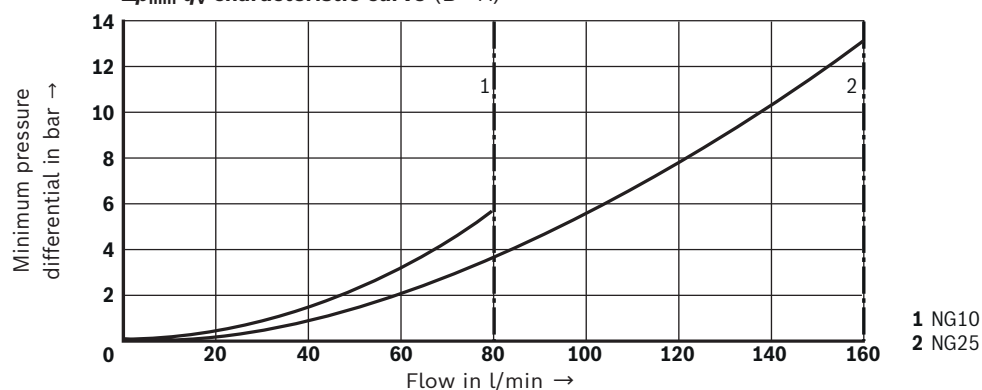
\Delta p_{min}-q_v characteristic curve (B→A)
