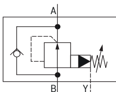
Subplate mounting "DR...Y"
