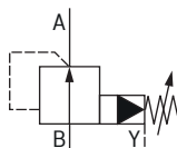
Subplate mounting; screw-in cartridge valve "DR...YM"; "DR . K...YM"
