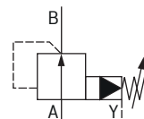
Threaded connection "DR . G...YM"
